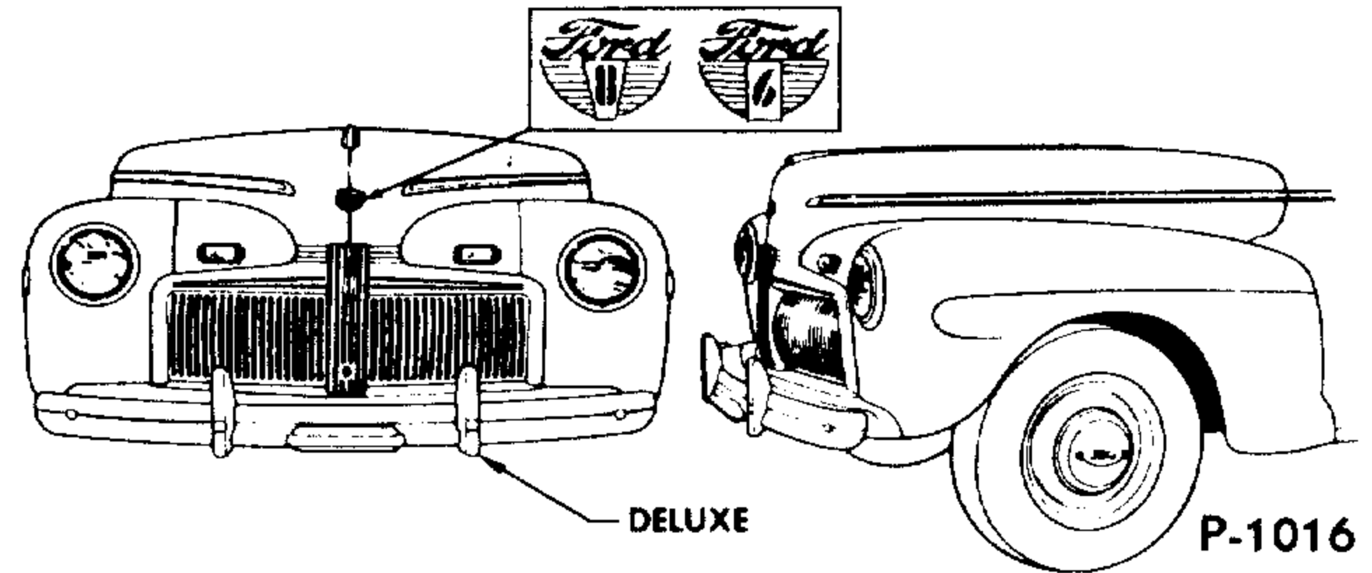
MODEL 21A FORD DELUXE 90 HP. 8-Cylinder Engine MODEL 2GA FORD DELUXE 90 HP. 6-Cylinder Engine (114" Wheelbase)
